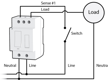
Latching
