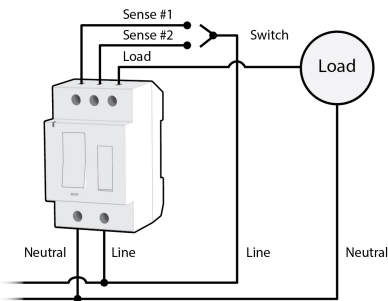
Dual Momentary
